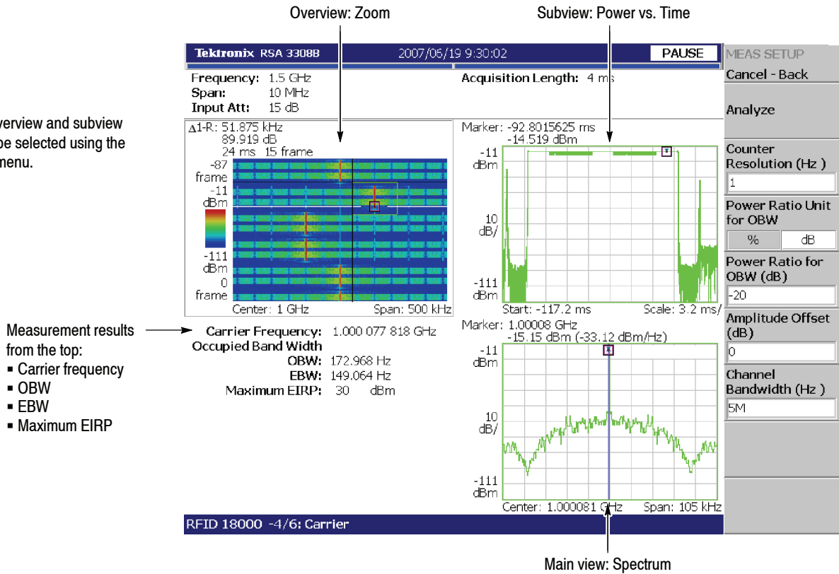
Figure 3-54: Carrier measurement
