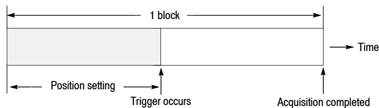
Figure 3- 104: Trigger position
