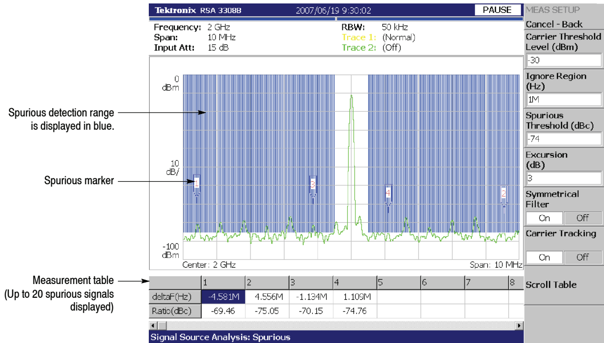
Figure 3-78: Spurious measurement
