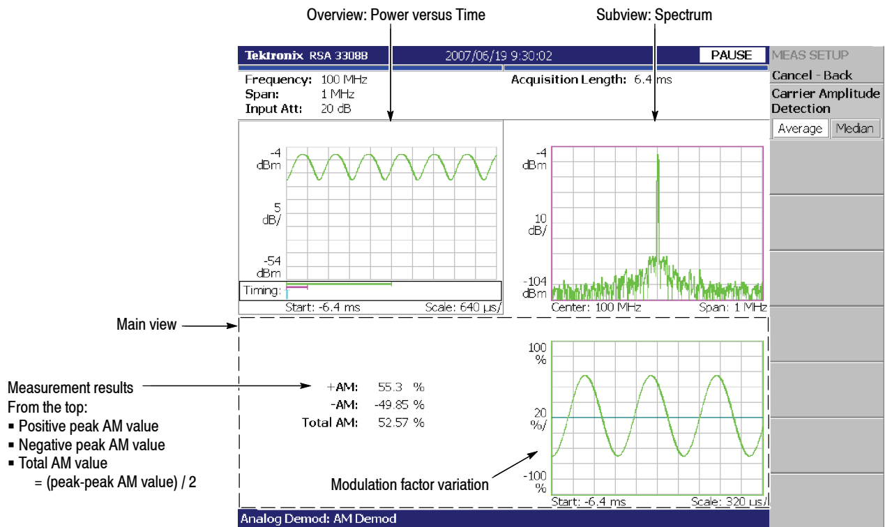
Figure 3-36: AM demod measurement
