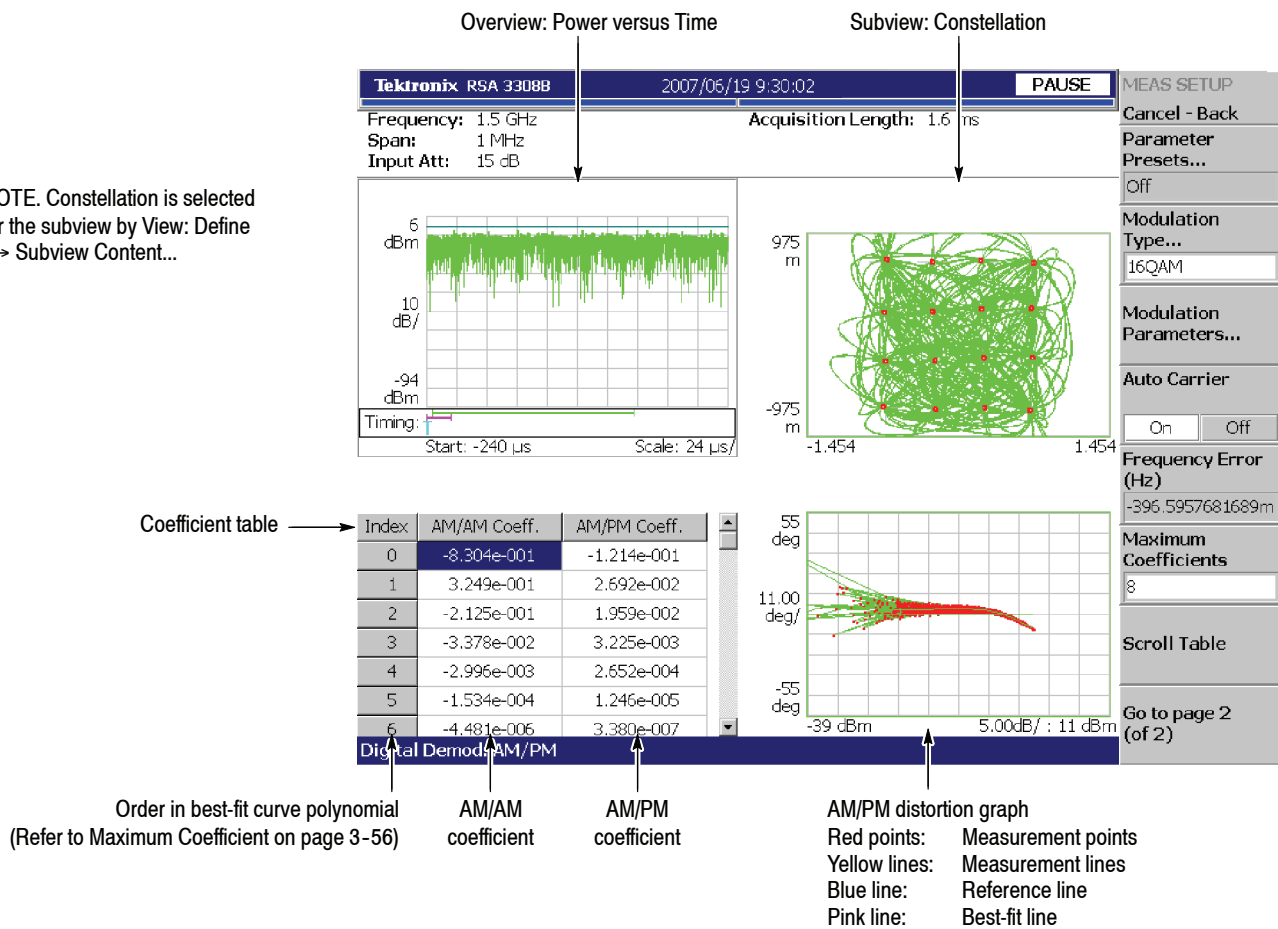
Figure 3-50: AM/PM measurement
