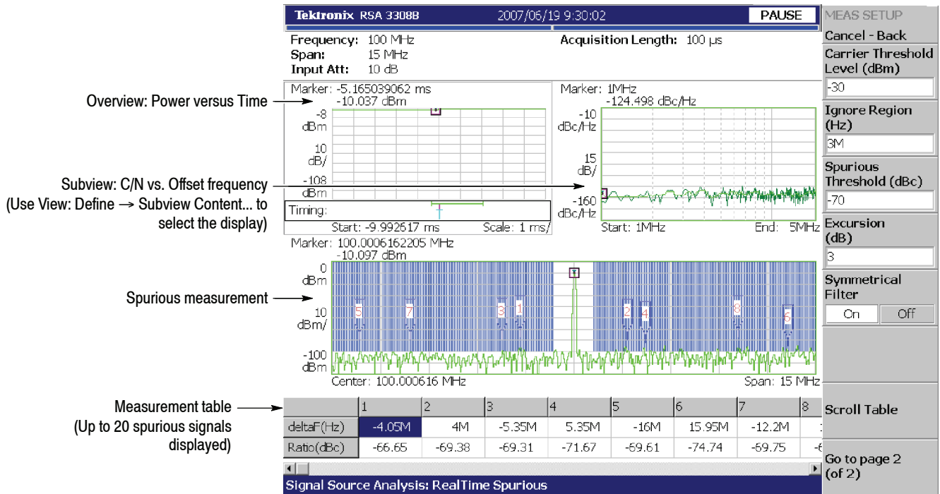
Figure 3-82: Real-time spurious measurement
