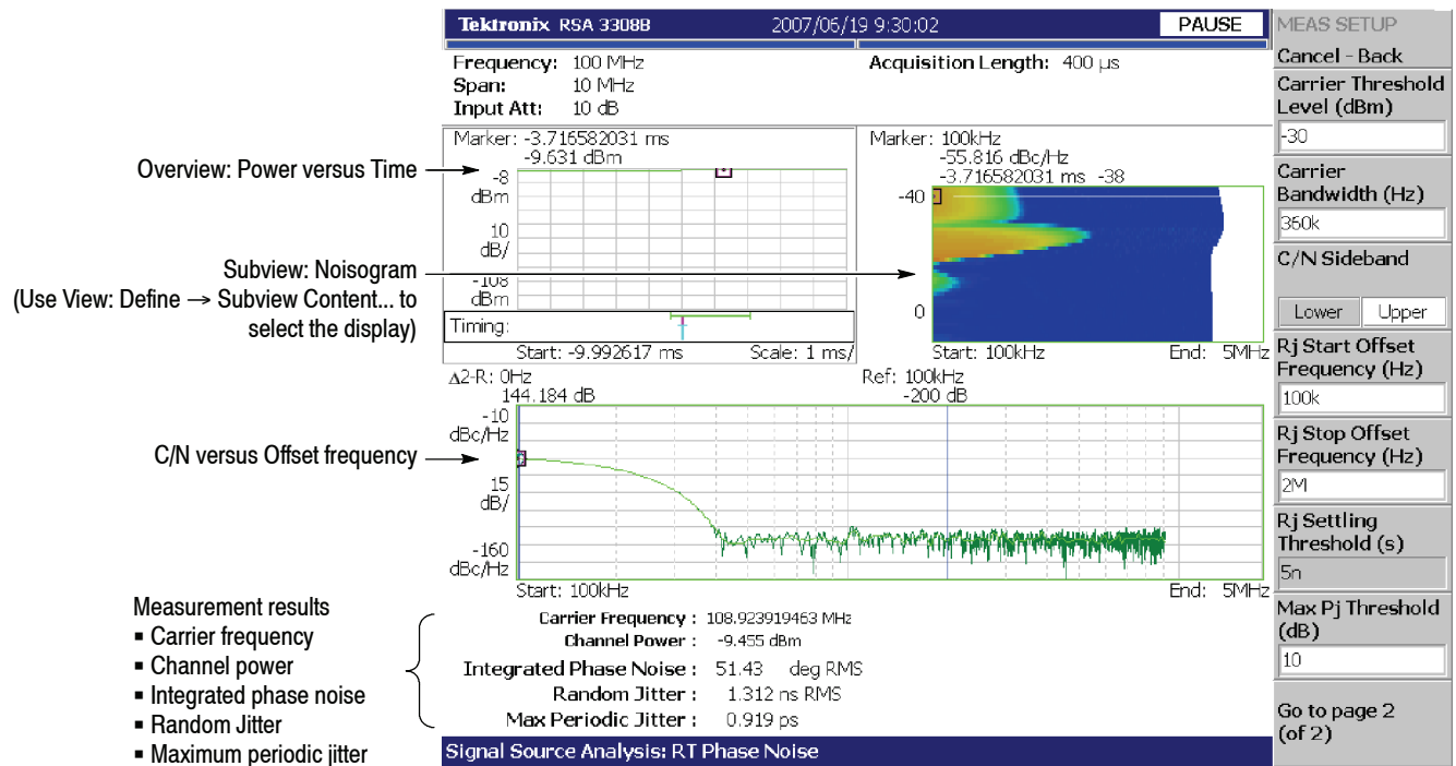
Figure 3-80: Real-time phase noise measurement
