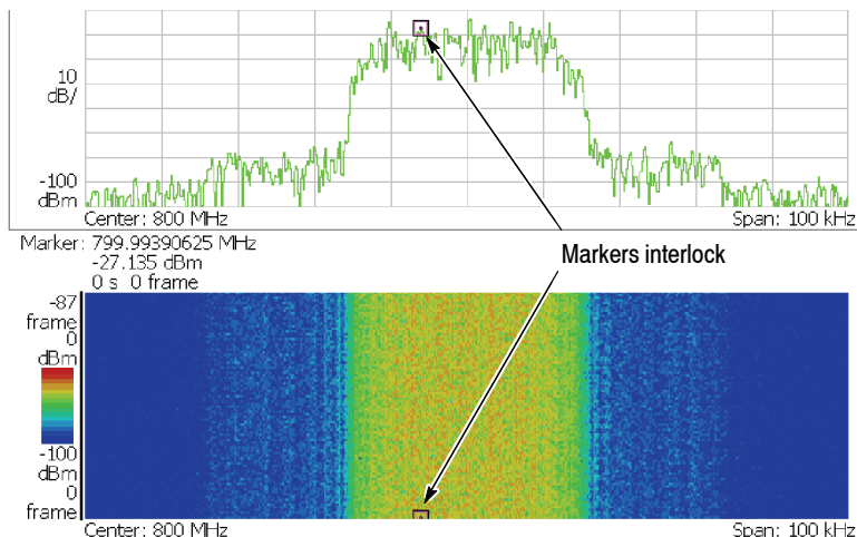
Figure 3- 157: Interlocked markers
