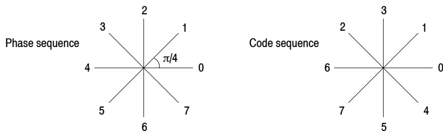
Figure 3- 139: D8PSK symbol value
