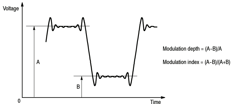
Figure 3-63: Definition of the modulation depth and index
