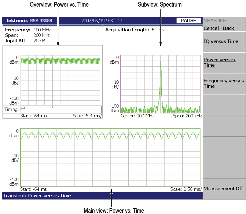
Figure 3-66: Power variance measurement
