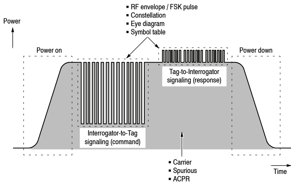
Figure 3-53: RFID waveform and measurement items
