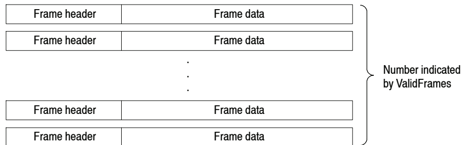
Figure 3- 175: Data block
