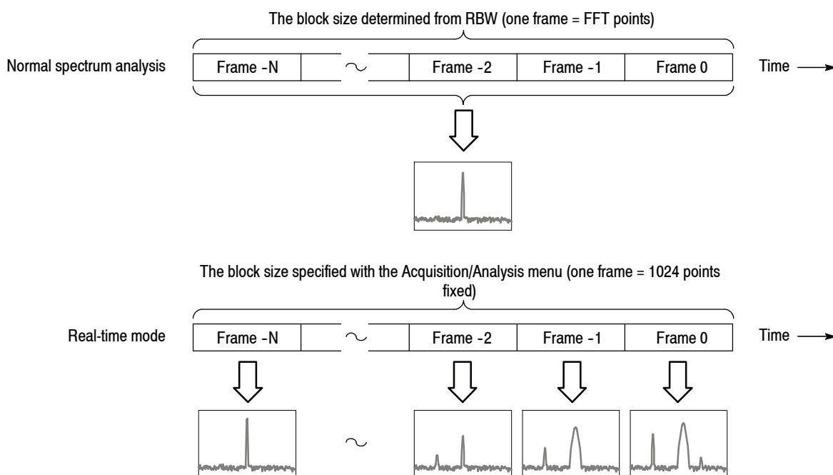
Figure 3-22: Difference between normal and real-time modes
