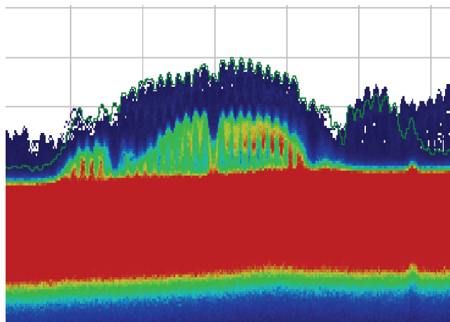
Figure 3-17: DPX spectrum display
