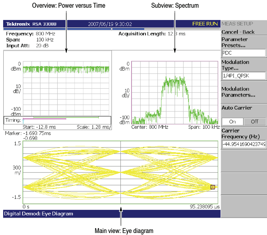
Figure 3-47: Eye diagram analysis
