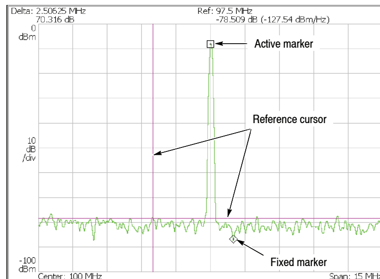
Figure 3-151: Marker display
