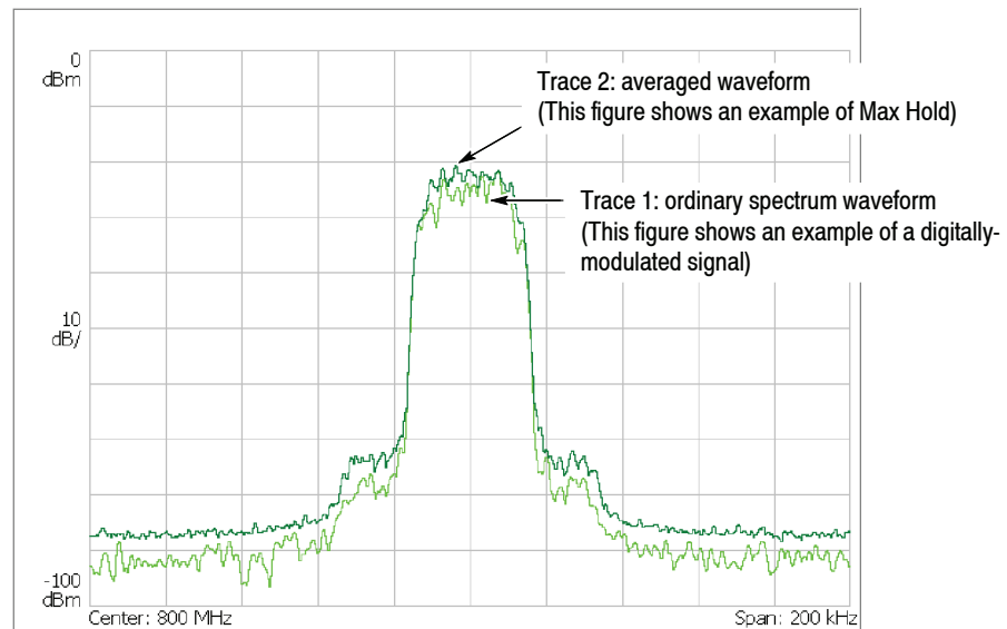
Figure 3- 126: Compared display
