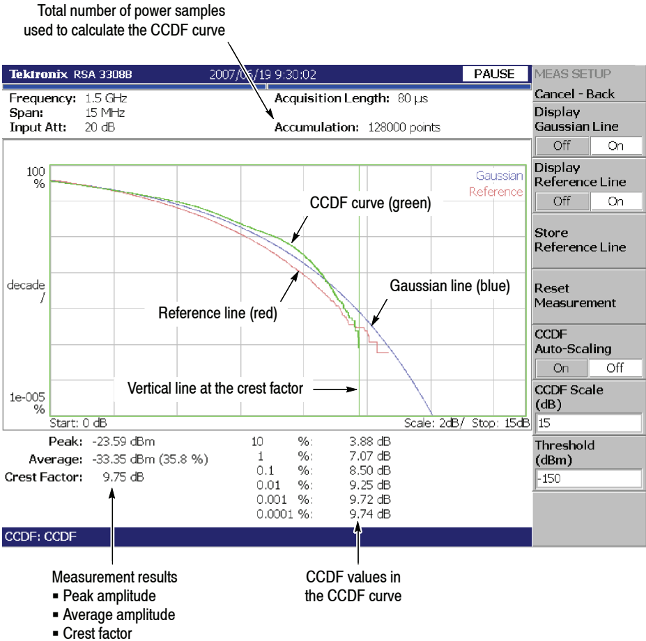
Figure 3-69: CCDF single view
