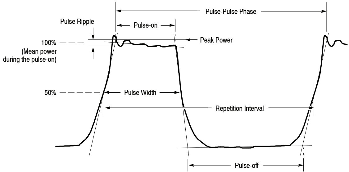
Figure 3-71: Definition of pulse characteristics
