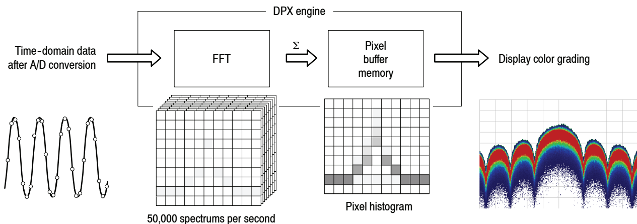
Figure 3-16: DPX process flow
