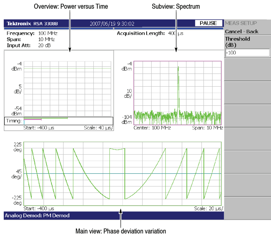
Figure 3-38: PM demod measurement
