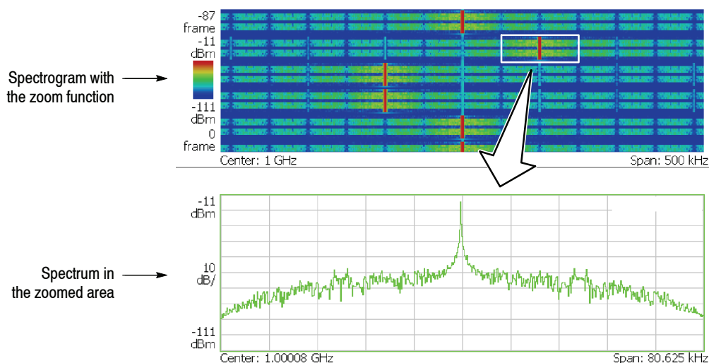
Figure 3-24: Zoom function
