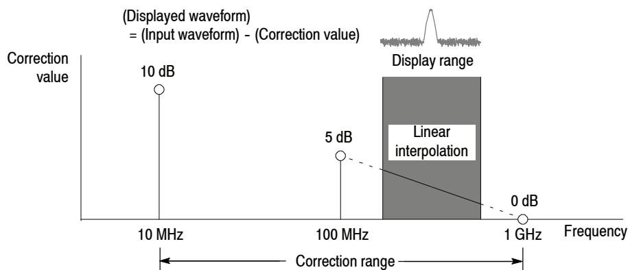
Figure 3-93: Amplitude correction example
