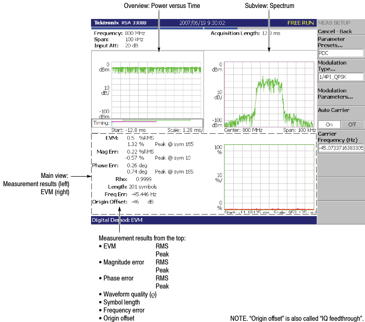
Figure 3-43: EVM measurement
