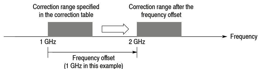
Figure 3-96: Frequency offset
