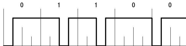
Figure 3-57: Modified Miller code
