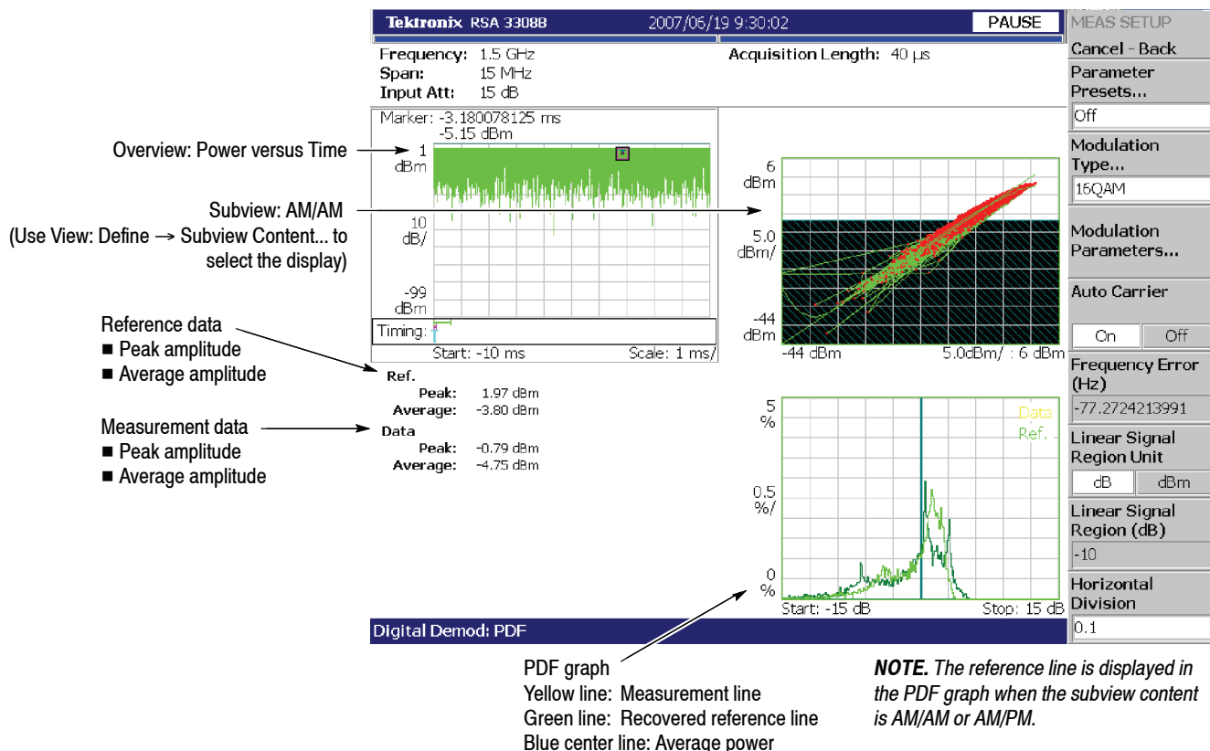
Figure 3-52: PDF measurement
