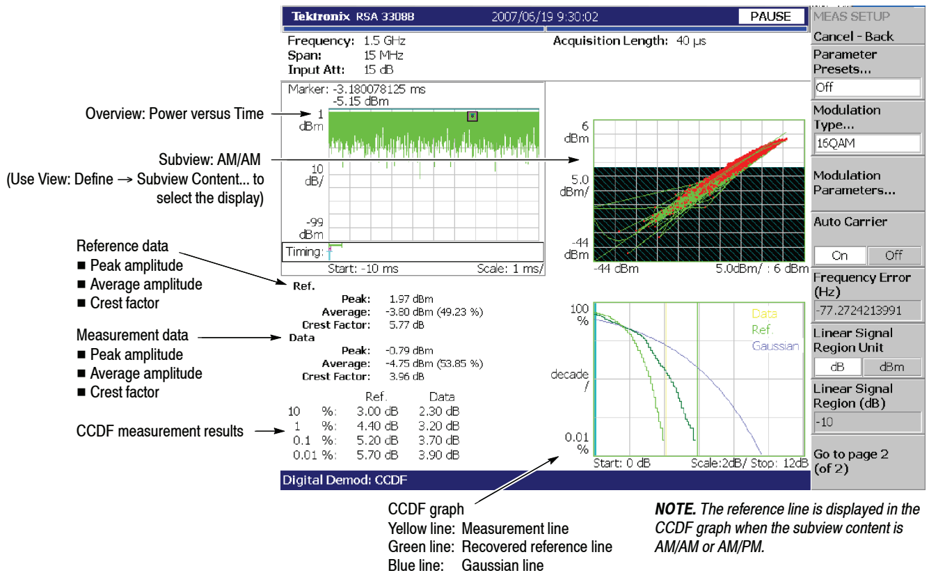
Figure 3-51: CCDF measurement
