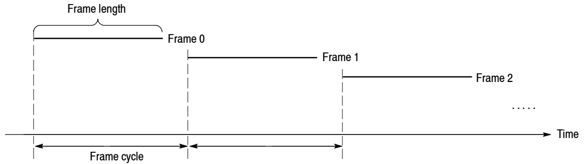
Figure 3-101: Frame cycle
