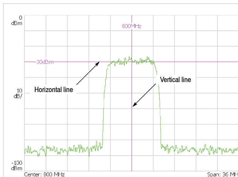
Figure 3-145: Display line
