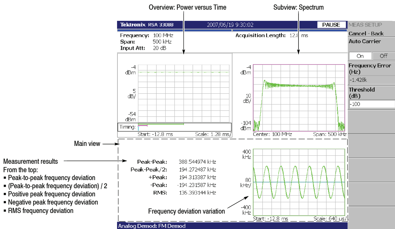
Figure 3-37: FM demod measurement
