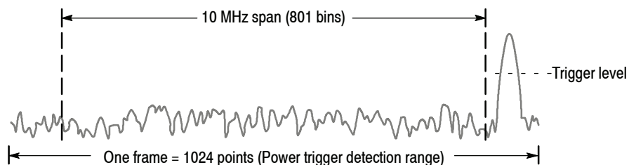
Figure 3-105: Power trigger detection range
