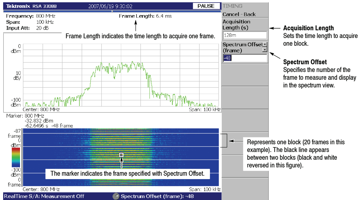
Figure 3-23: Real-time mode
