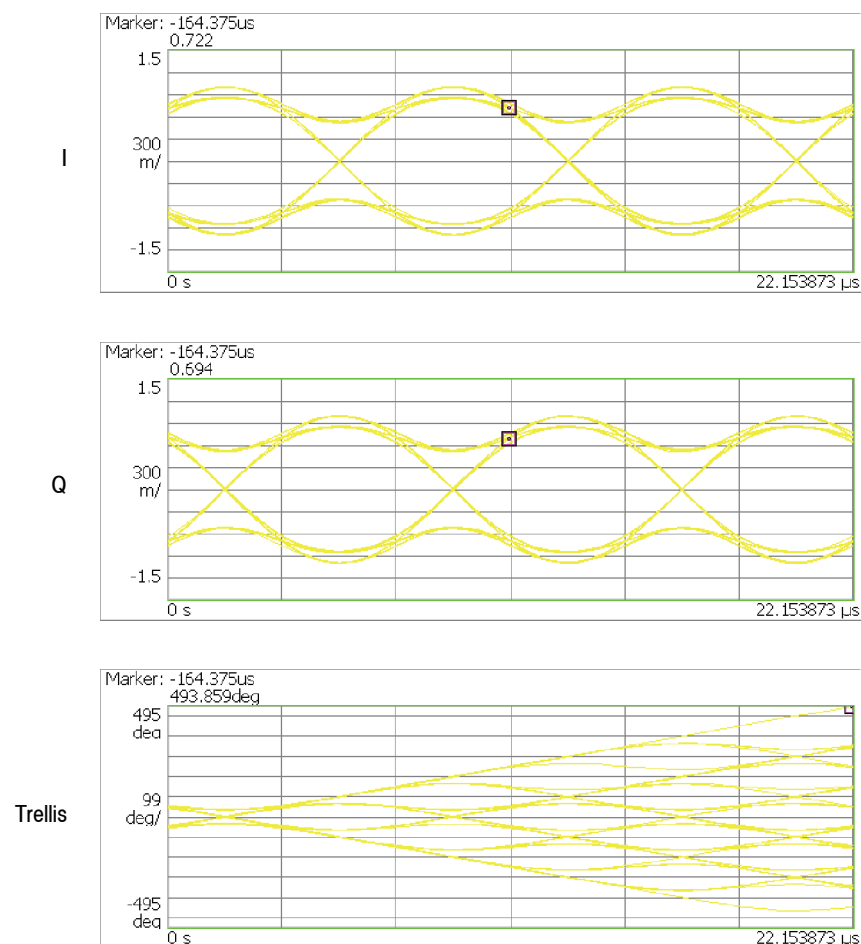
Figure 3-140: Eye diagram view
