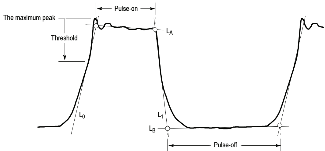
Figure 3-72: Definition of pulse-on/off
