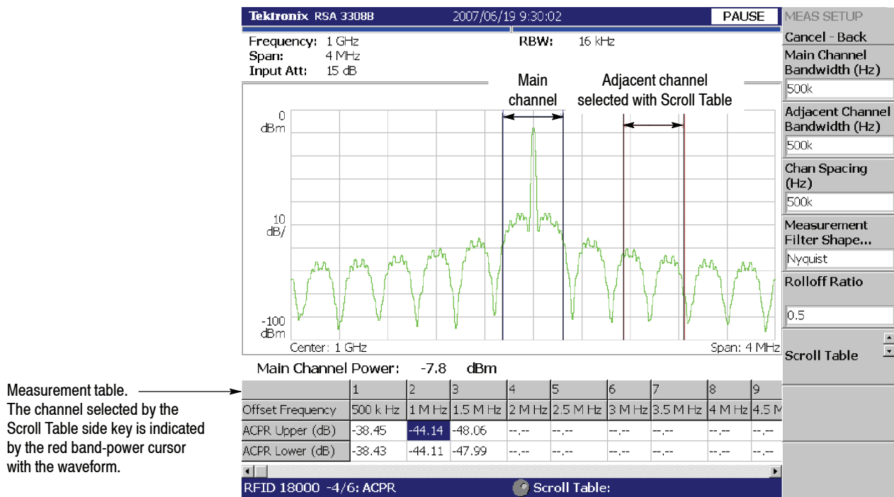
Figure 3-56: ACPR measurements
