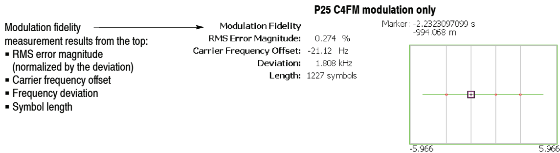
Figure 3-42: Constellation analysis
