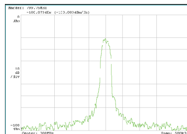
Figure 3-21: Single display
