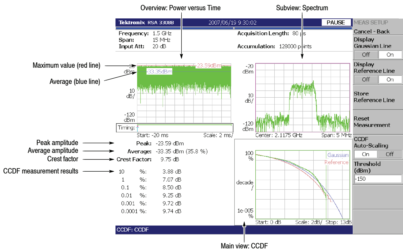
Figure 3-70: CCDF multi-view
