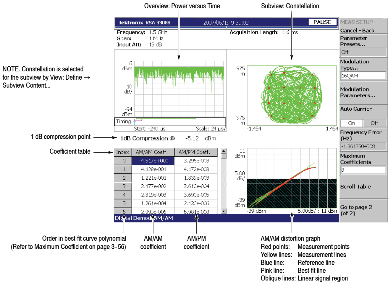
Figure 3-49: AM/AM measurement
