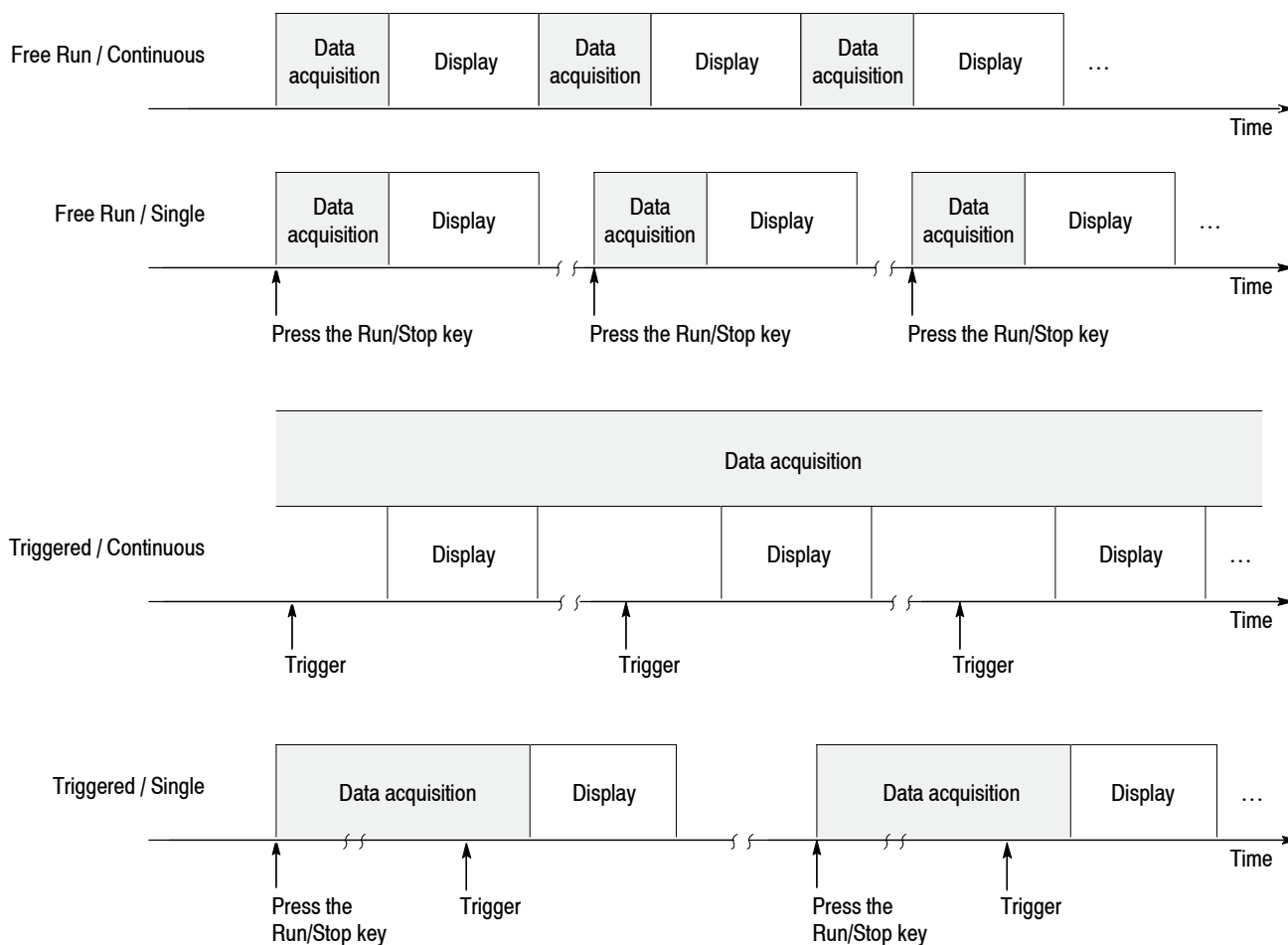
Figure 3-107: Acquiring and displaying data by Trigger and Repeat modes
