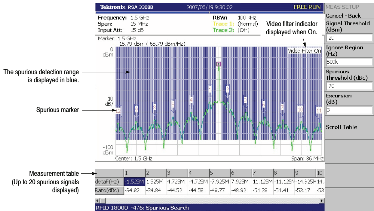
Figure 3-55: Spurious measurement
