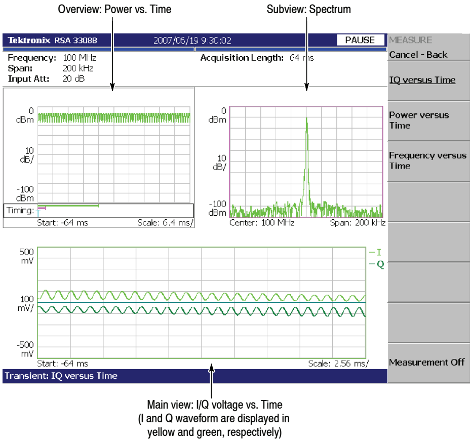
Figure 3-65: IQ versus Time measurement
