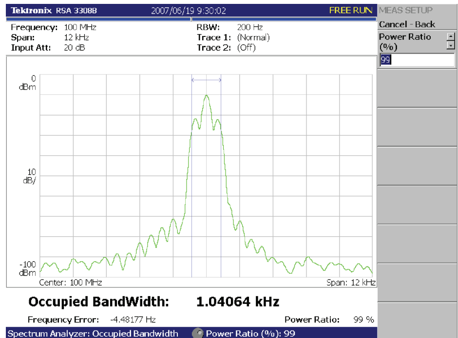
Figure 3-10: OBW measurement
