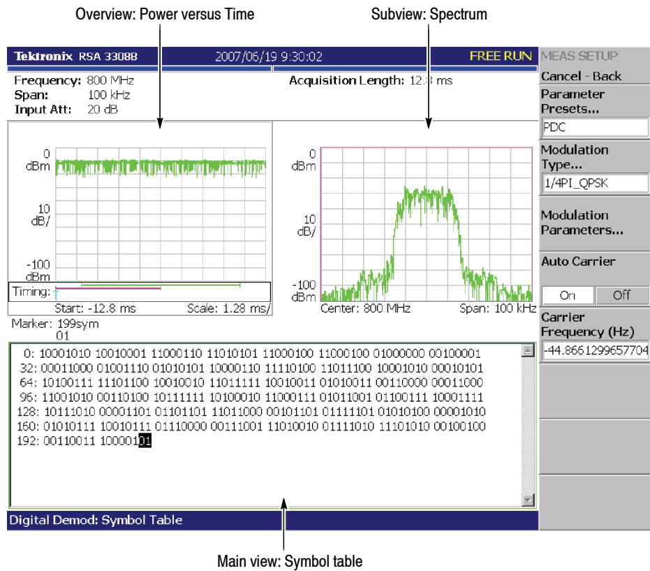
Figure 3-46: Symbol table analysis
