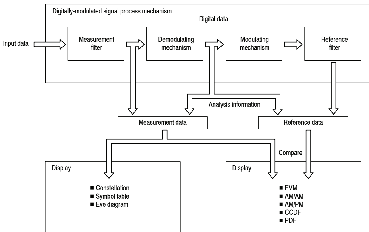
Figure 3-41: Process flow for digitally-modulated signals
