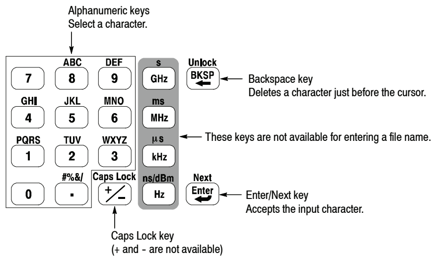
Figure 3- 172: Alphanumeric keypad
