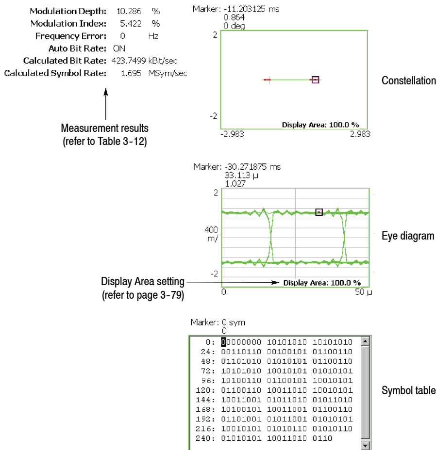
Figure 3-62: Constellation, eye diagram, and symbol table (main view)
