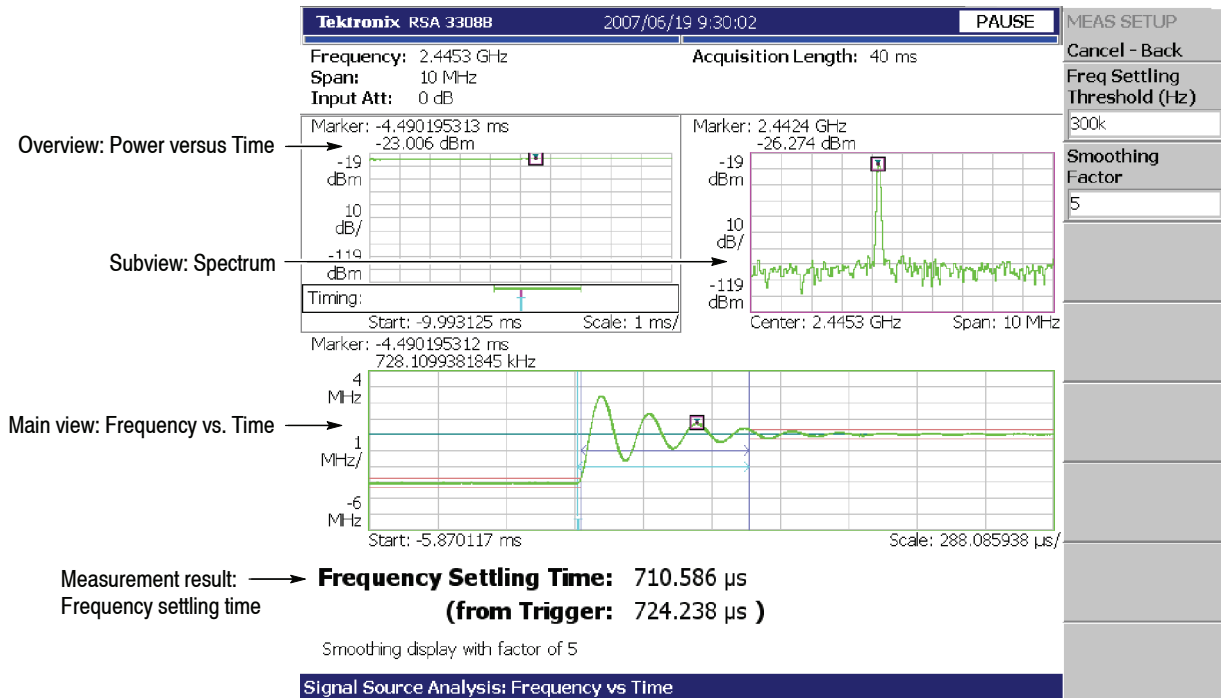
Figure 3-84: Frequency versus Time measurement
