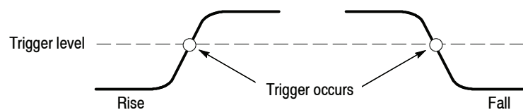
Figure 3- 106: Trigger level and slope
