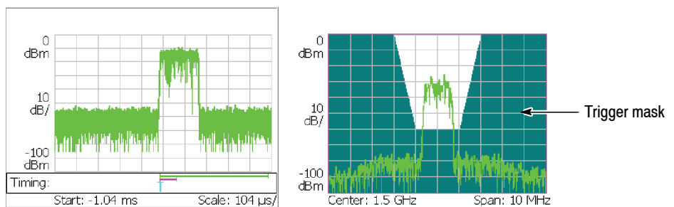
Figure 3-108: Trigger mask
