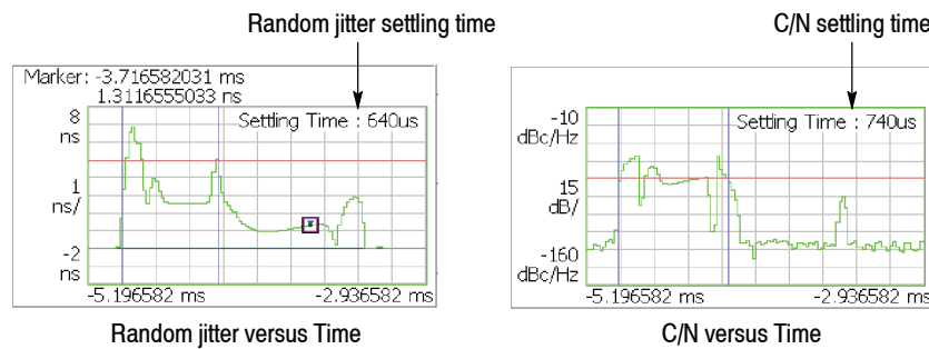
Figure 3-81: Settling time displayed in the subview
