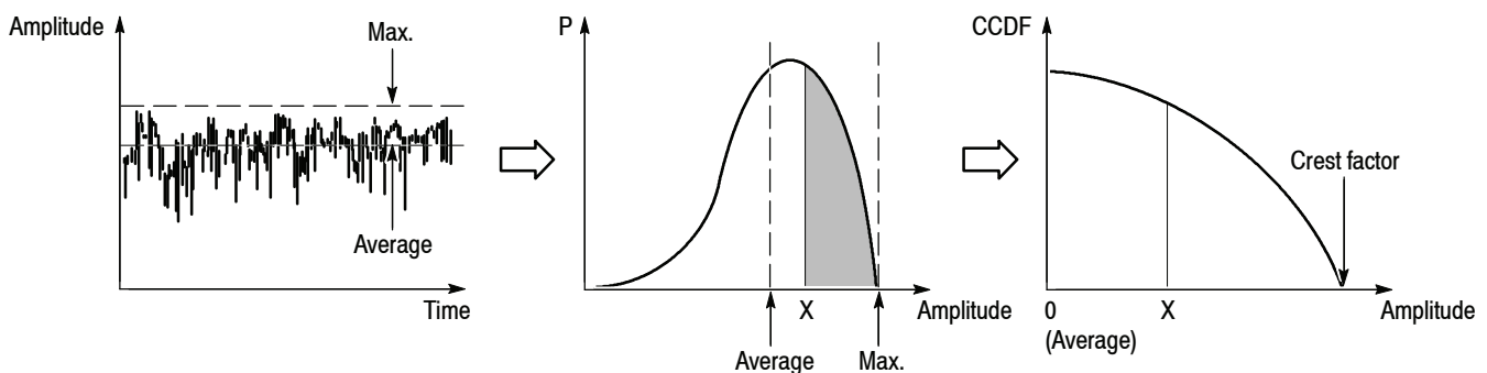
Figure 3-68: CCDF calculation process
