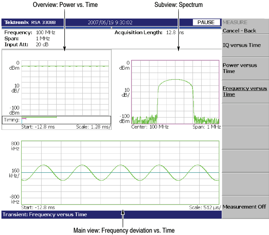
Figure 3-67: Frequency measurement
