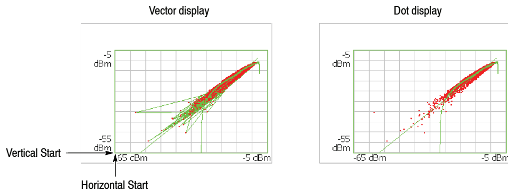
Figure 3-141: Vector and dot displays for AM/AM view
