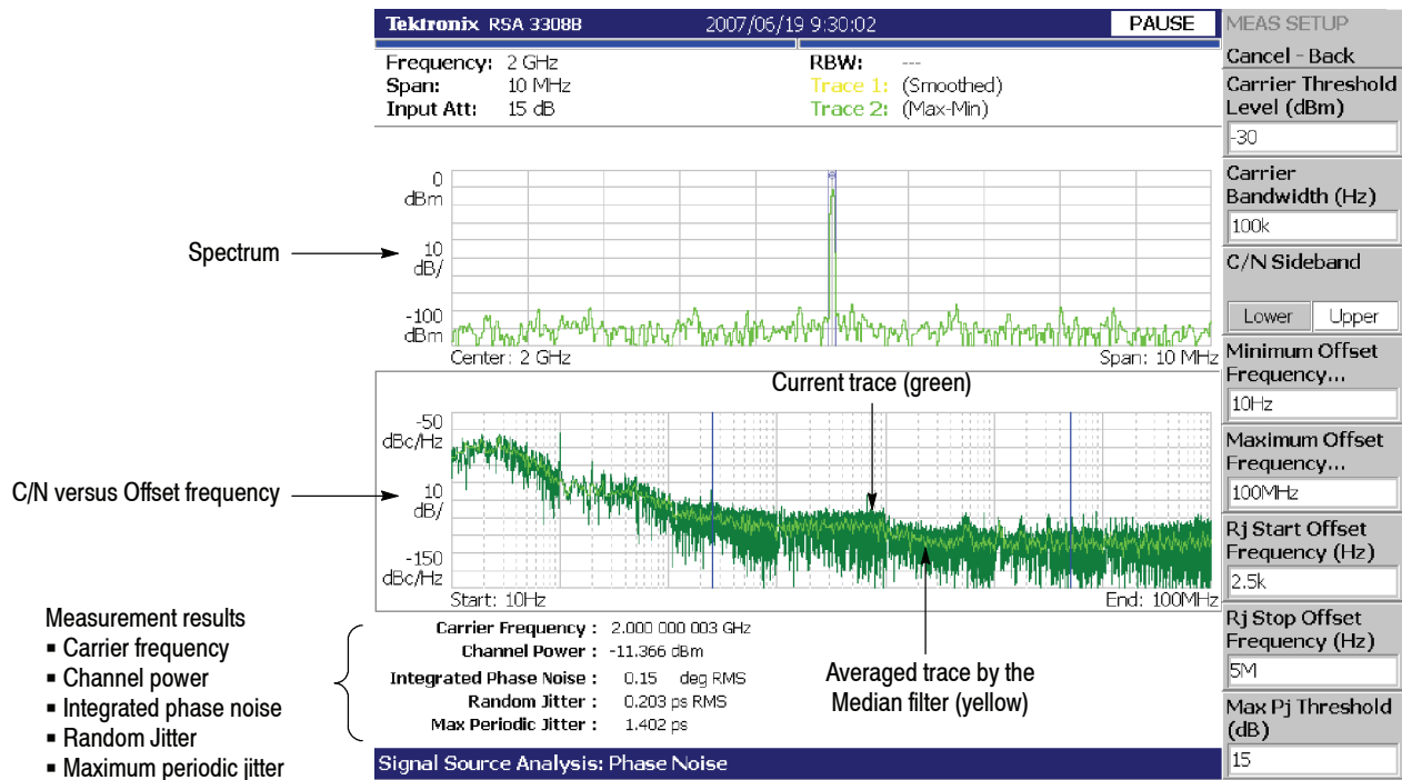
Figure 3-77: Phase noise measurement
